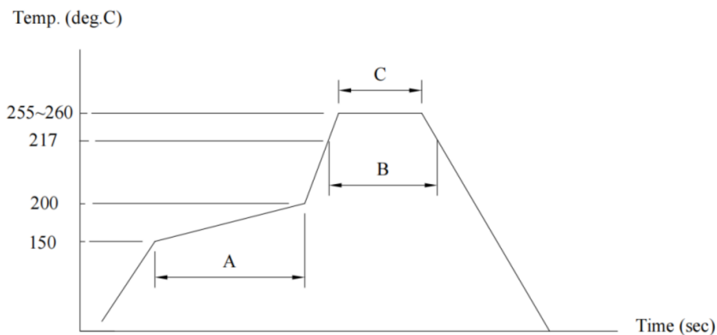
Figure 6. Reflow Profile
