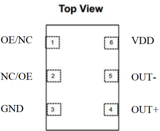
Figure 5 Pin Assignments
