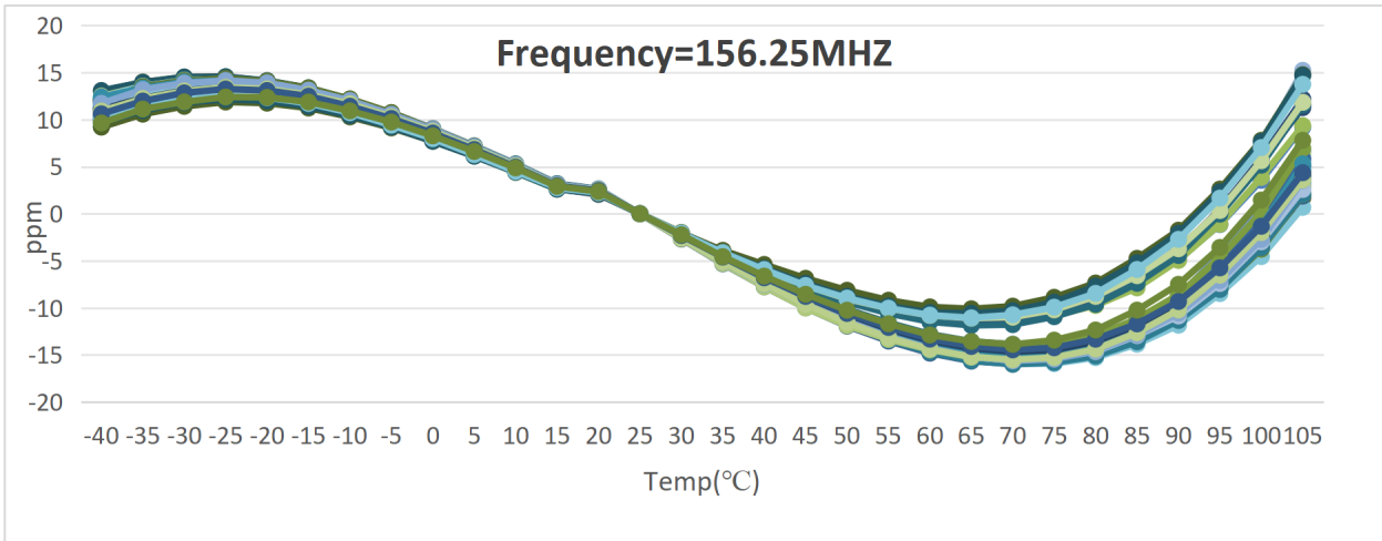
Figure 4 Frequency vsTemperature
