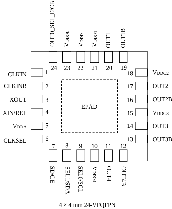
Figure 2. 24-VFQFPN Pin Assignment, 4.0mm x 4.0mm x 0.9mm, 0.5mm Pitch (Top view)
