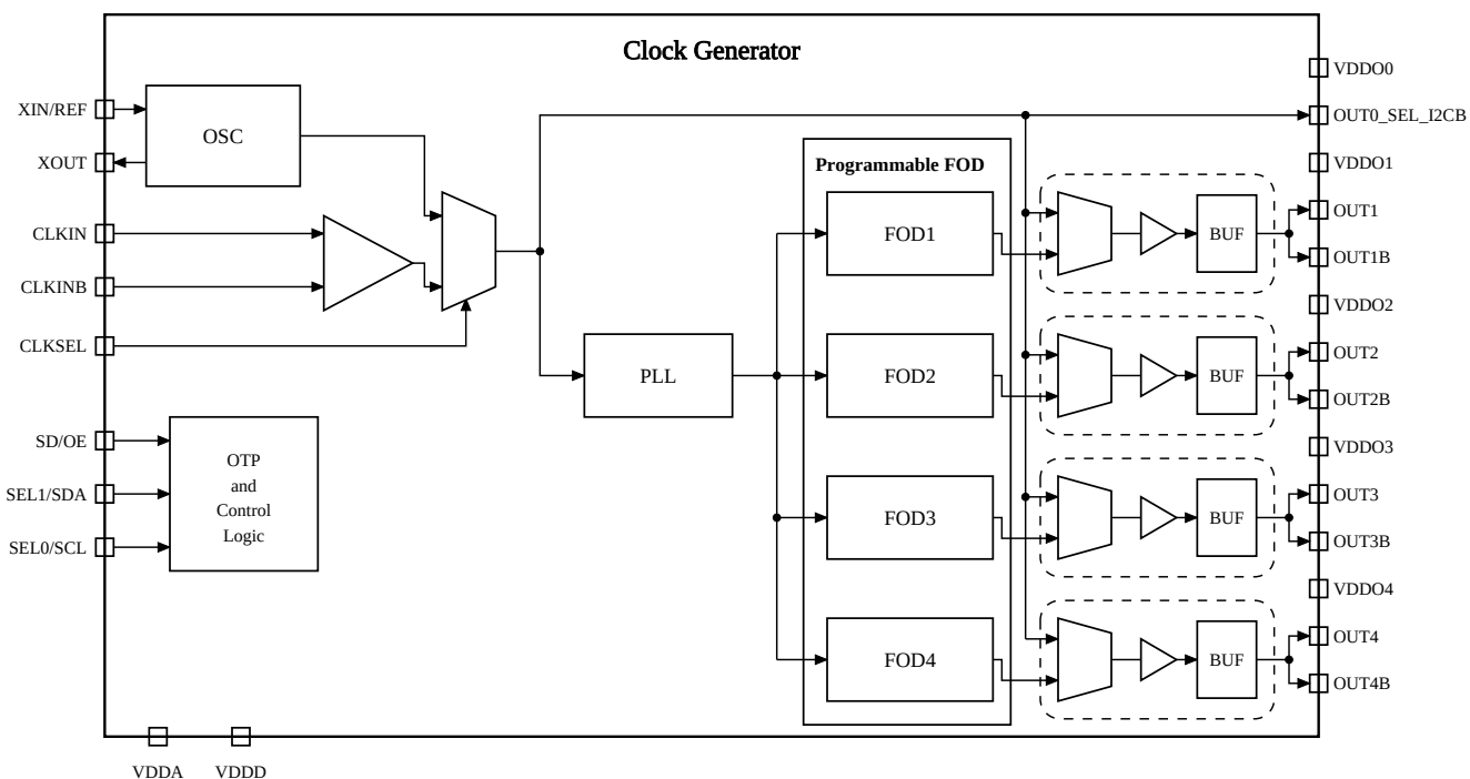
Figure 1. SYKG6965 Block Diagram
