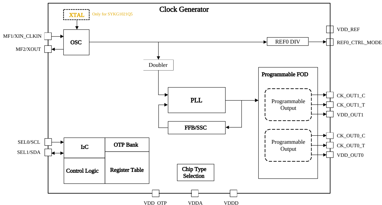
Figure 1. SYKG1021E/Q5 Block Diagram
