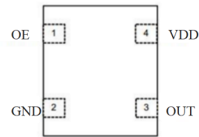
Figure 3 Pin Assignments
