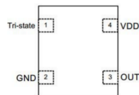
Pin Assignments
