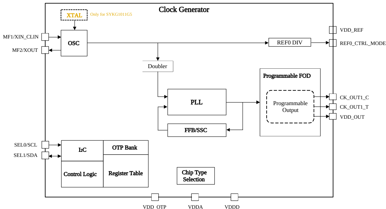
Figure 1. SYKG1011E/Q5 Block Diagram
