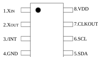
YSN8563S (SOP-8)
