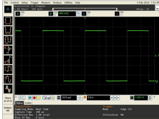
Figure 3. LVCMOS Output Swing (V dd =1.8V)
